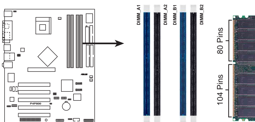
P4P800 184-Pin DDR DIMM Sockets
