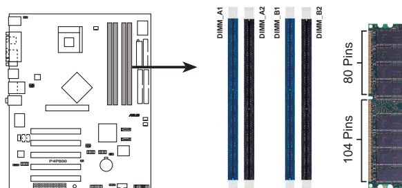
P4P800 184-Pin DDR DIMM Sockets
