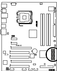
P5K-E SATA connectors
