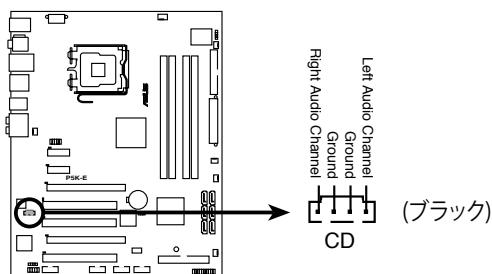
P5K-E Internal audio connector
