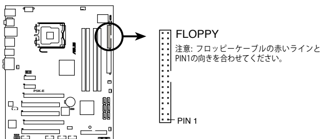
P5K-E Floppy disk drive connector
